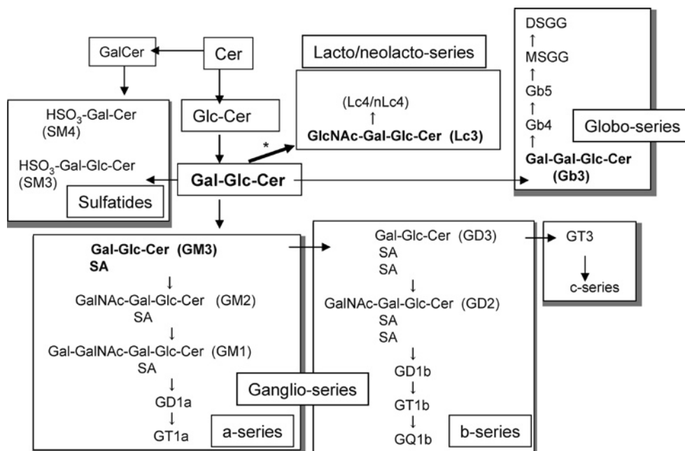
Fig. 1 Synthetic pathway of glycosphingolipids. Majority of glycosphingolipids are synthesized via GlcCer (and LacCer), while a minor portion is via GalCer. SA, N-acetyl-neuraminic acid. GlcCer, glucosylceramide; LacCer, lactosylceramide; GalCer, galactosylceramide. \beta 3Gn-T5 catalyzes conversion of LacCer to Lc3.
